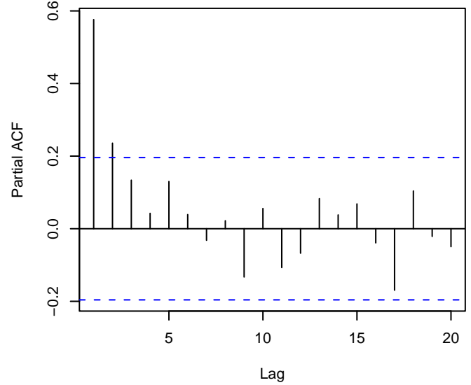
Series diff(y4)
