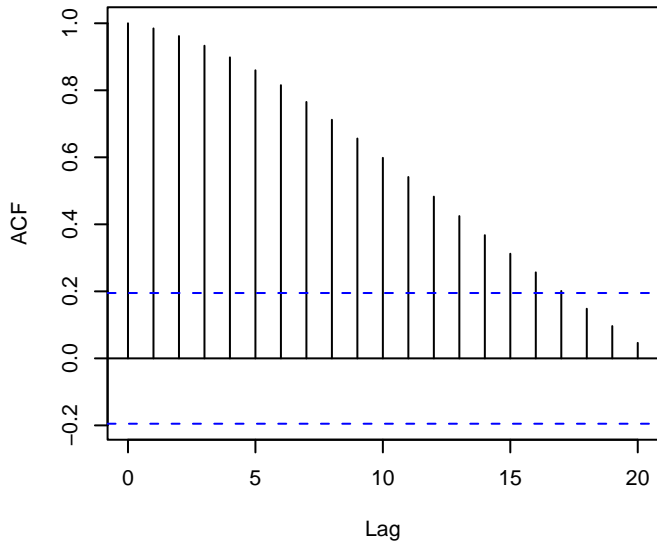
Series y4
