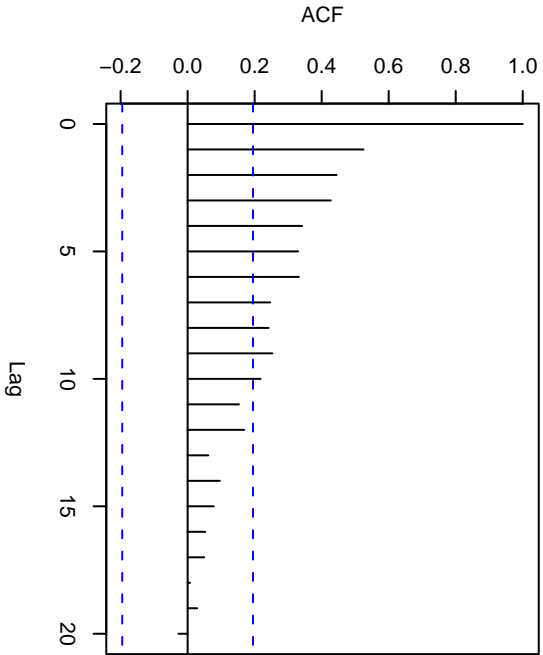
Series y1
