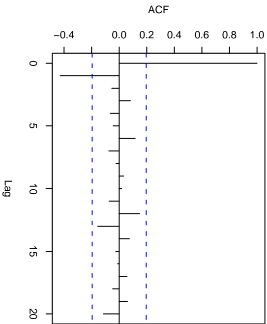
Series diff(y1)
