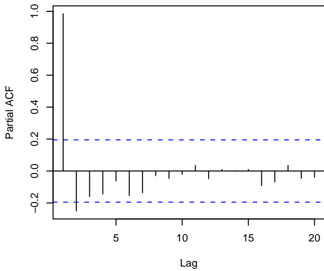
Series y4
