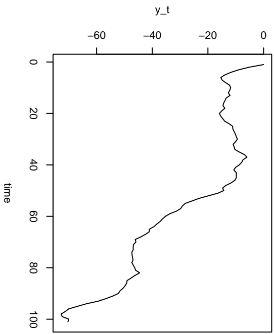
ARIMA(1,1,0)
