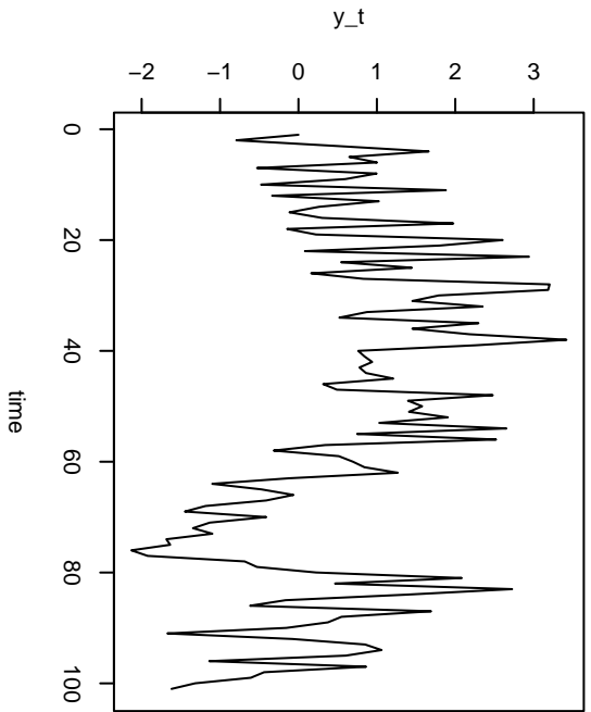
ARIMA(0,1,1)
