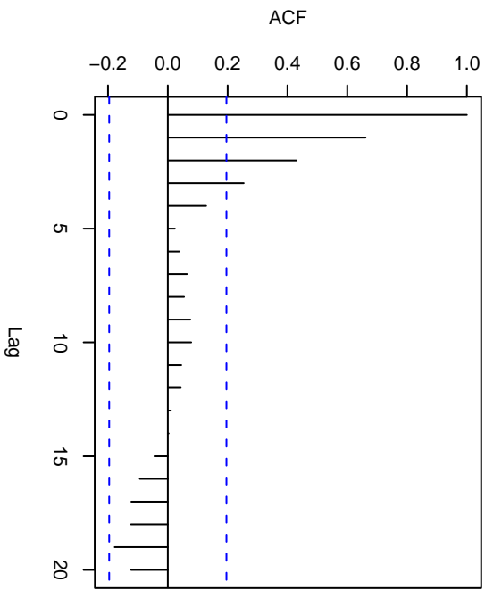
Series diff(y3)
