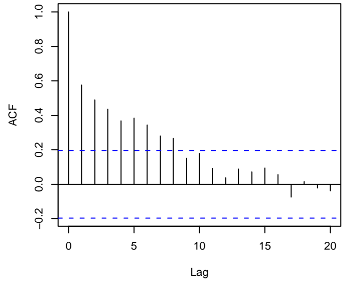
Series diff(y4)
